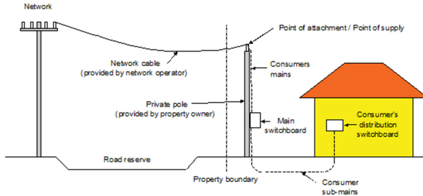
Figure 2: Overhead connection to Consumer Pole and underground connection to Property.
